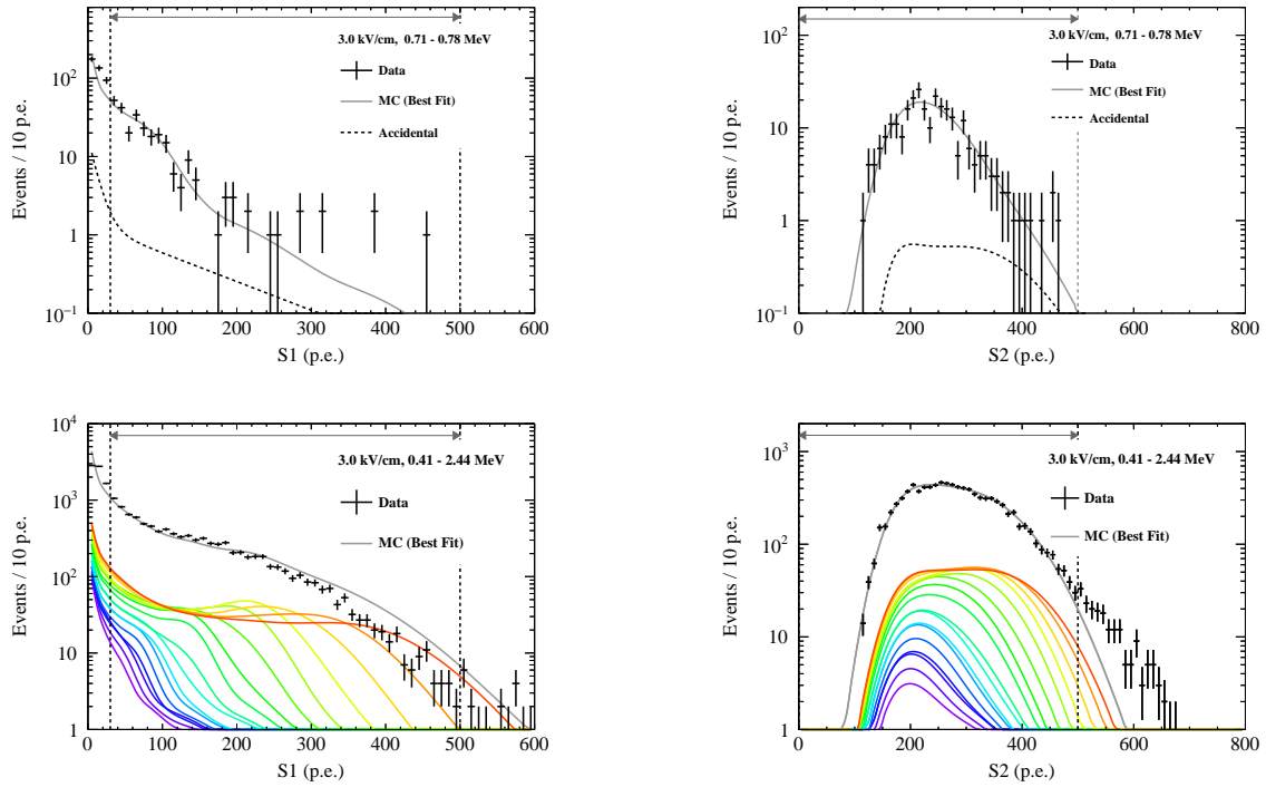
Fig. 5.25. The S1 (left) and S2 (right) spectra taken at the electric field of 3.0 kV/cm and MC-derived spectra simultaneously fitted to experimental data. The figure descriptions are the same as in Fig. 5.21.
