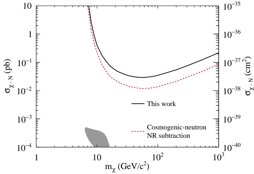
Fig. 8.11. Expected WIMP-nucleon cross section 90% C.L. upper limits by subtracting the cosmic-ray induced NR events (red dashed line). The black solid line is the same as in Fig. 7.23
