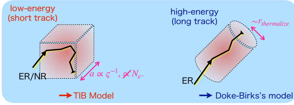
Fig. 3.3. Schematic illustration of an interpretation of the two recombination models with respect to the recoiled particle track length.
