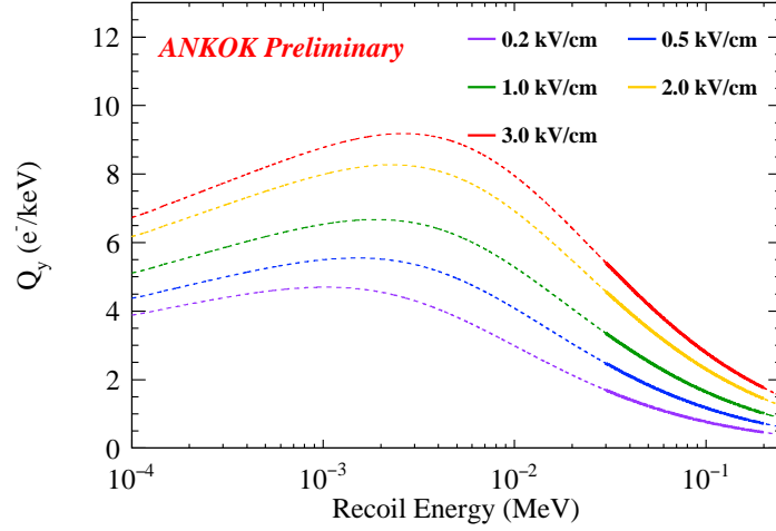
Fig. 5.31. Ionization yield for NR as a function of recoil energy derived from the model function. The colored solid lines represent the energy threshold of this analysis, and the corresponding dashed lines are extrapolations.
