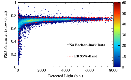
Fig. 6.5. Distribution of the PSD parameter (“slow/total”) versus the observed light signal. The data requires the back-to-back tagging described in Section 6.3.3. The red dashed lines correspond to the 95% containing band for ER events.
