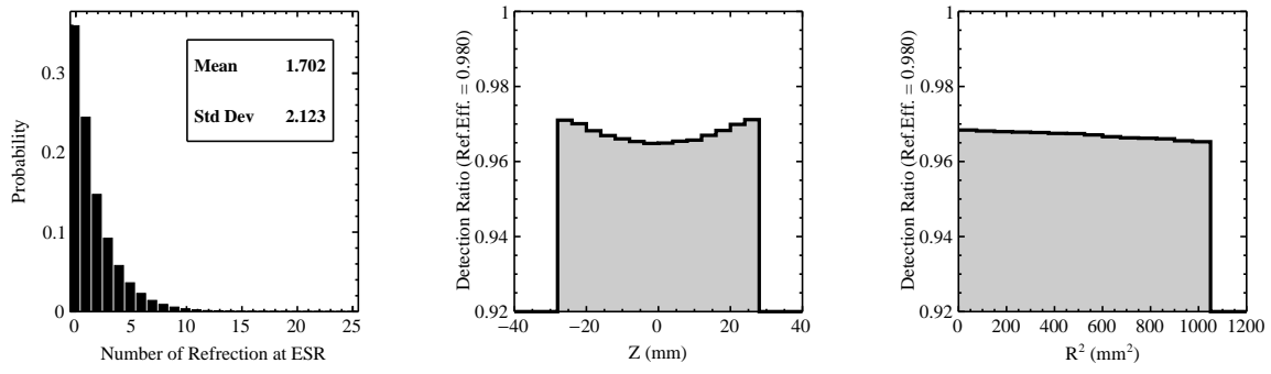
Fig. 4.18. Average number of reflection (left) and the transportation efficiency as a function of the initial position (center and right) computed from the toy MC.
