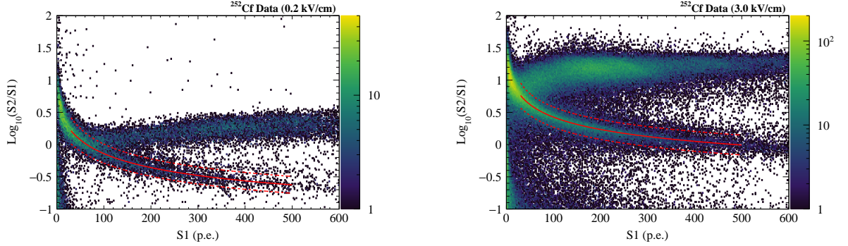
Fig. 5.13. The \log_{10}(S2/S1) distributions as a function of S1 yield taken under electric fields of 0.2 (left) and 3.0 kV/cm (right) without the PSD cut. Two dashed lines in each panel correspond to the band for \log_{10}(S2/S1) cut ( \pm 2\sigma ).
