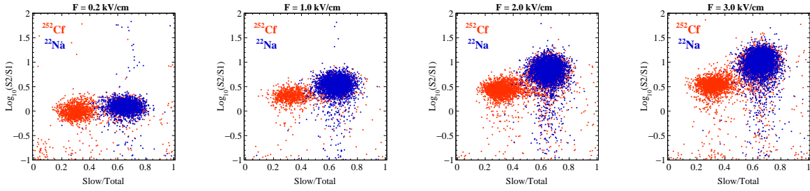
Fig. 3.15. Distributions of ^{252}\text{Cf} (both NR and ER) and ^{22}\text{Na} (ER) events of approximately 10 \text{keV}_{\text{ee}} at fields of 0.2, 1.0, 2.0, and 3.0 \text{kV/cm} (from left to right) in the PSD parameter versus the ionization to scintillation ratio.
