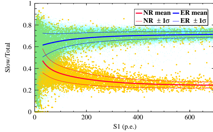
Fig. 3.13. Distributions of ^{252}\text{Cf} (both NR and ER) and ^{22}\text{Na} (ER) events at null field in S1 versus slow/total plain, where S1 of 50 p.e. corresponds to approximately 5 \text{keV}_{\text{ee}} . The thick and thin lines represent the NR (red) and ER (blue) bands of \pm 1\sigma .
