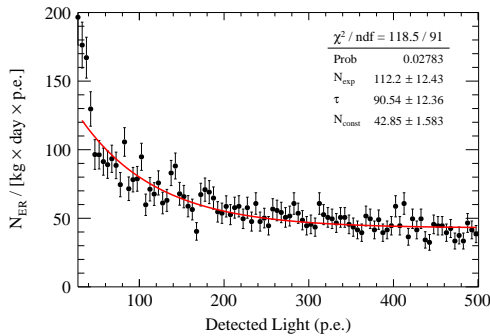
Fig. 7.18. ER spectrum evaluated by the same data used in the WIMP search. The red line is an empirical model function.
