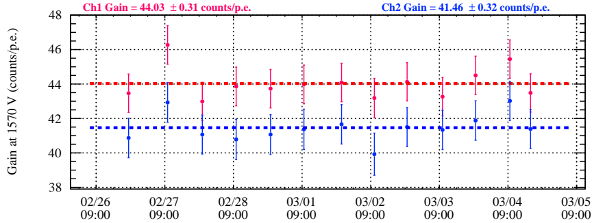
Fig. 6.3. Time evolution of the gain of the two PMTs calibrated with the LED. The error bar of each point includes both statistical and systematical uncertainties.
