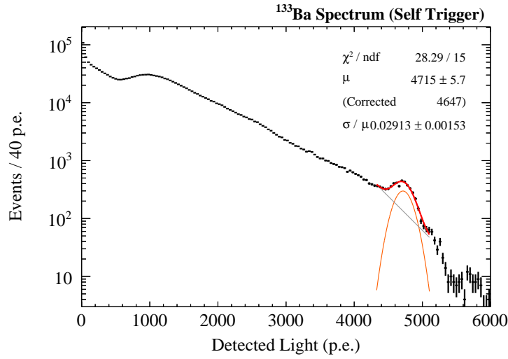
Fig. 6.8. The observed light spectrum from the ^{133}\text{Ba} source. The red line represents the fit function.
