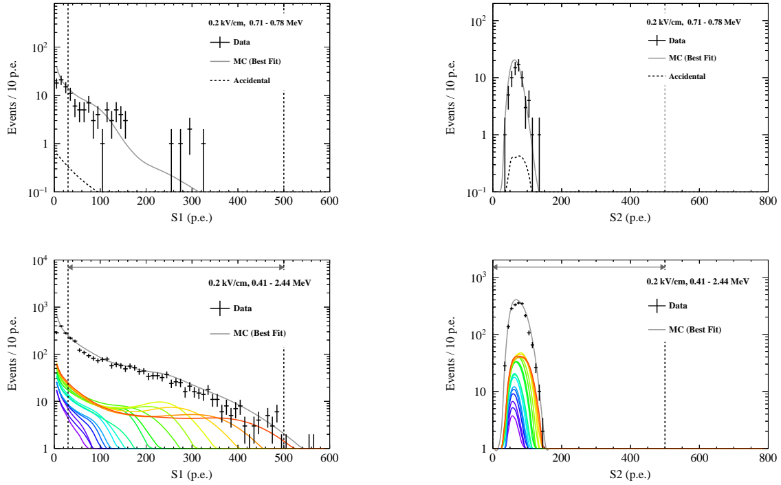
Fig. 5.21. Top: S1 (left) and S2 (right) spectra of the NR data sample taken at the electric field of 0.2 kV/cm and MC-derived spectra simultaneously fitted to experimental data for TOF in the range of 79–83 ns (corresponding to a neutron energy of about 0.75 MeV). The areas indicated by vertical dashed lines and gray arrow represent the fitting range. Bottom: The S1 (left) and S2 (right) spectra for entire TOF range of interest. The figure descriptions are the same as in Fig. 5.20.
