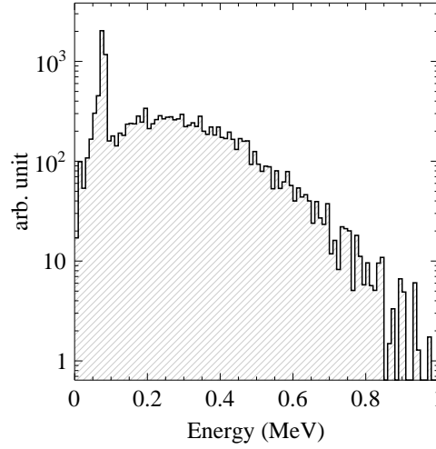
Fig. 7.7. Relative intensity of x-ray from ^{210}\text{Pb} and its daughter calculated using PHITS simulation.
