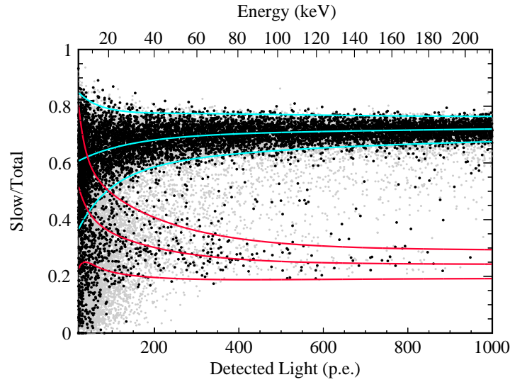
Fig. 7.21. Distribution of the events surviving all event selections (black point) in the detected light versus slow/total plane. The gray point represents the event surviving all selections but anti-veto coincidence. Also shown are the mean and 2\sigma bands for ER and NR, respectively.
