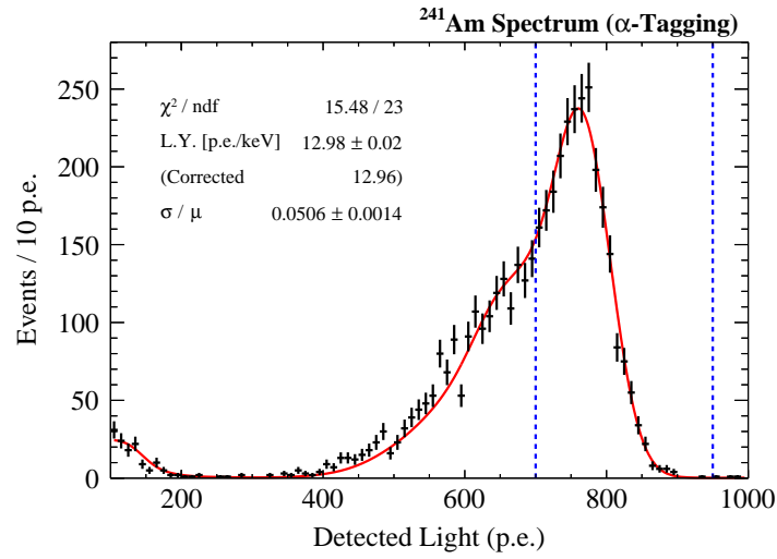
Fig. 6.16. The observed light spectrum from the ^{241}\text{Am} source by requiring \alpha -ray detection by the veto PMTs, along with the MC fit spectrum (red line). The blue dashed vertical lines represent the fitting range.
