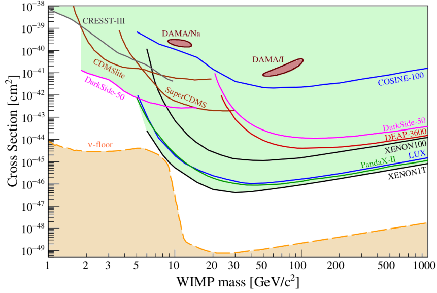
Fig. 2.7. A compilation of direct detection experiments on WIMP mass and cross section parameter space. The solid curves are the 90% upper limit from each experiments, and the two contours are the interpretation of DAMA annual modulation signature. The dashed curve represents an approximate limit of the sensitivity of direct detection experiments where irreducible background from solar, atmospheric, and diffuse supernova neutrinos elastic scattering (CEvNS) events will be seen (neutrino floor). Original figure is taken from Ref. [18].
