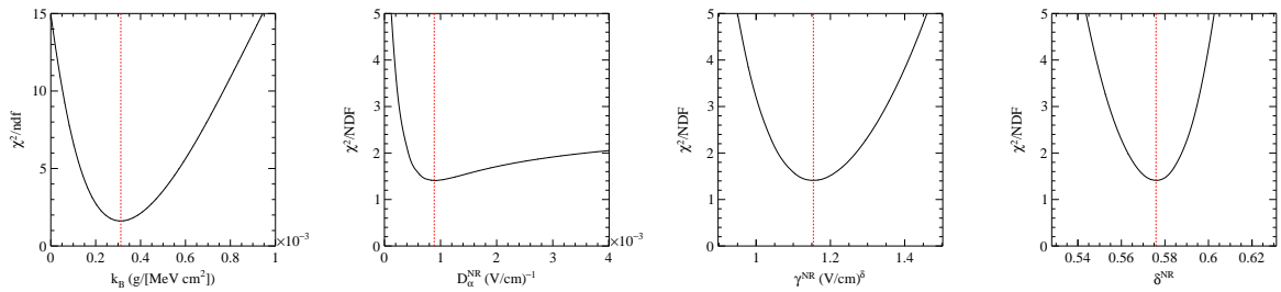
Fig. 5.27. Distributions of \chi^2/ndf of each parameter ( k_B , D_\alpha^{NR} , \gamma^{NR} , and \delta^{NR} from left to right) in the simultaneous fit. The vertical red dashed lines represent the best-fit values.
