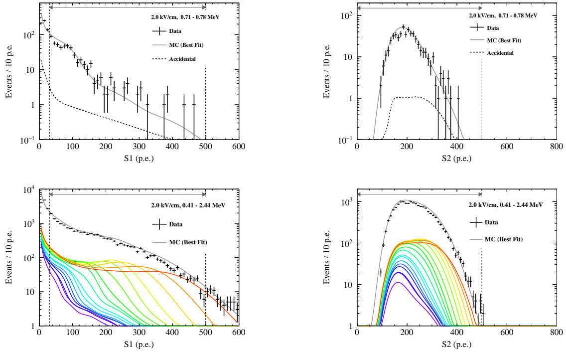
Fig. 5.24. The S1 (left) and S2 (right) spectra taken at the electric field of 2.0 kV/cm and MC-derived spectra simultaneously fitted to experimental data. The figure descriptions are the same as in Fig. 5.21.
