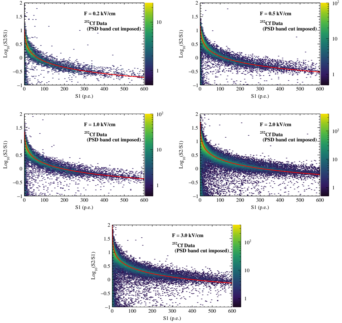
Fig. 5.28. The ^{252}\text{Cf} data taken with the electric fields of 0.2, 0.5, 1.0, 2.0, and 3.0 kV/cm (from left to right and top to bottom) in \log_{10}(S2/S1) versus the S1 plane, overlaid with the prediction from the NR model and the best fit parameters (solid line).
