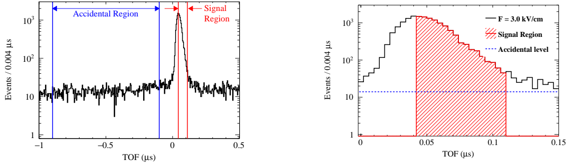
Fig. 5.14. TOF distribution and definition of the signal and accidental regions. The accidental contamination is estimated from \text{TOF} = -0.9 – -0.1 \mu\text{s} , as shown in the left panel, and the level of the accidental events is represented as the dashed line in the right panel. The data shown is taken at F = 3.0 \text{ kV/cm} .
