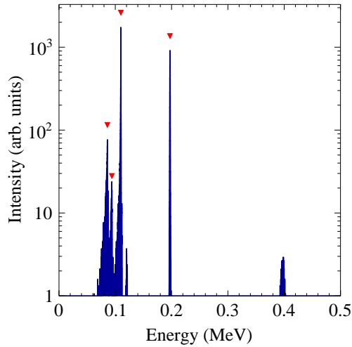
Fig. 6.9. The \gamma -ray energy spectrum from (n, n'\gamma) reaction in ^{19}\text{F} induced by ^{252}\text{Cf} fast neutron based on PHITS [108]. The red markers indicate the energies of 85.9, 93.9, 109.8, and 197.1 keV based on a peak-finding algorithm.
