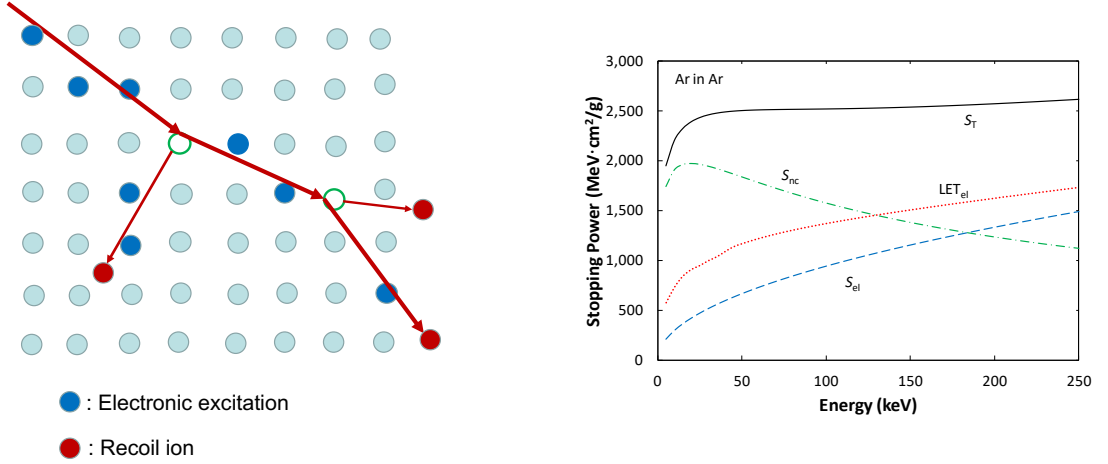
Fig. 3.2. Left: schematic illustration of the collision cascade from the recoiled nuclei travelling the detector medium. The recoiled nuclear losses its energy through elastic or inelastic scattering leaving ionized or excited atoms. Right: calculated stopping power for NR in liquid argon as a function of recoil energy based on Lindhard theory. The lines with S_{nc} and S_{el} represent the stopping power (energy deposition per unit length on the incident particle) given to elastic (electronic) and inelastic (nuclear) processes, respectively, while the S_T is the sum of them. The red line ( \text{LET}_{el} ) represents the electronic linear energy transfer, which gathers contributions from every secondaries and gives the energy used to produce excitation and ionization along the track. The figures are taken from Ref. [41].
