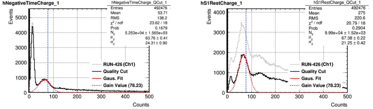
Fig. 5.10. Charge distributions and Gaussian fittings of pre-trigger (left) and S1-tail (right) regions.
