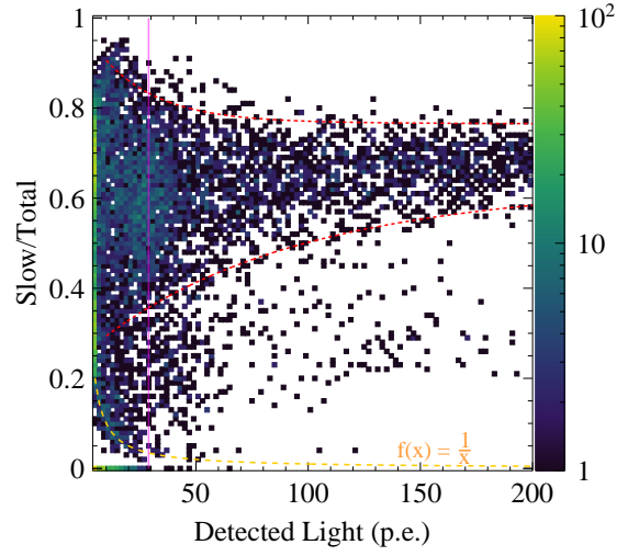
Fig. 6.18. Distribution of the PSD parameter versus the observed light signal. The orange dashed curve corresponds to events that have only 1 p.e. slow component, for reference. Events inside the red dashed lines are selected. The vertical magenta line corresponds to the ^{37}\text{Ar} peak.
