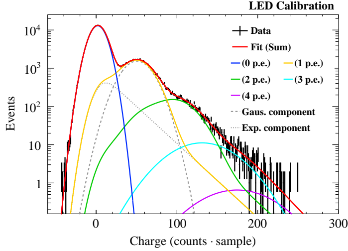
Fig. 6.2. A typical low-light charge distribution of a fiducial-viewing PMT from an LED calibration run. The charge is represented in units of integrated digitizer count (count · samples), where 1 count · sample corresponds to 9.8 \times 10^{-15} C. The solid red line is the model fit as expressed in Eq.(6.1), and the colored lines represent its components. The dashed and dotted lines indicate the Gaussian and exponential terms of the single photoelectron response.
