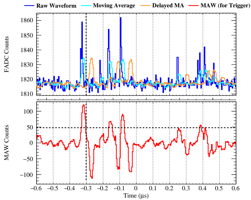
Fig. 4.8. Emulation of the FIR filter inside the FADC board. The MAW waveform, shown in bottom panel, is used for trigger decision. The horizontal dashed line represents a typical 1 p.e. threshold, and the vertical dashed lines represent the trigger timing in this case.
