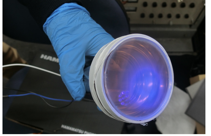
Fig. 4.5. Left: picture of TPB in the crucible used in the vacuum evaporation. Right: picture of the TPB-coated R11065 PMT, illuminated with an ultraviolet light.
