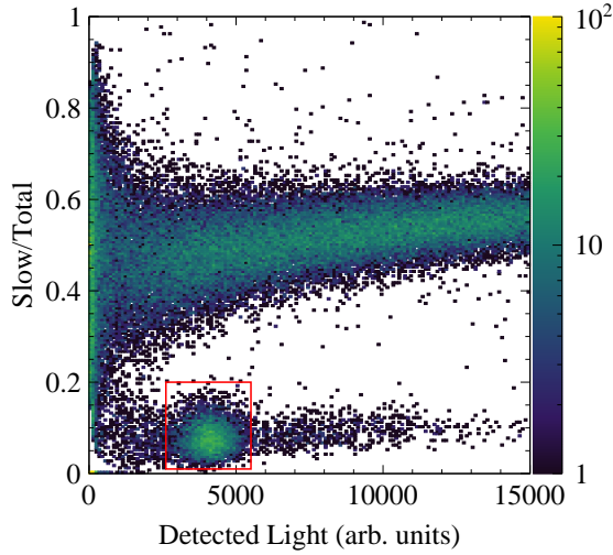
Fig. 6.14. Left: distribution of the observed signal by outer-bath PMTs in the detected-light versus PSD plain. The ^{241}\text{Am} region is defined to select the \alpha -ray tagging signal. Right: observed spectrum in fiducial before and after requiring the \alpha -ray signal inside the red box.
